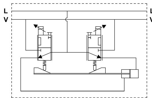
Hydraulic scheme
