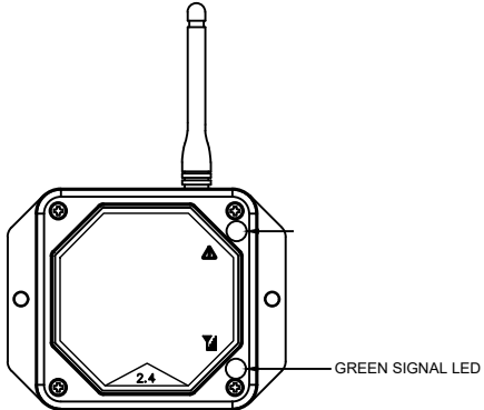
FIG. 1:RECEIVER FRONT
