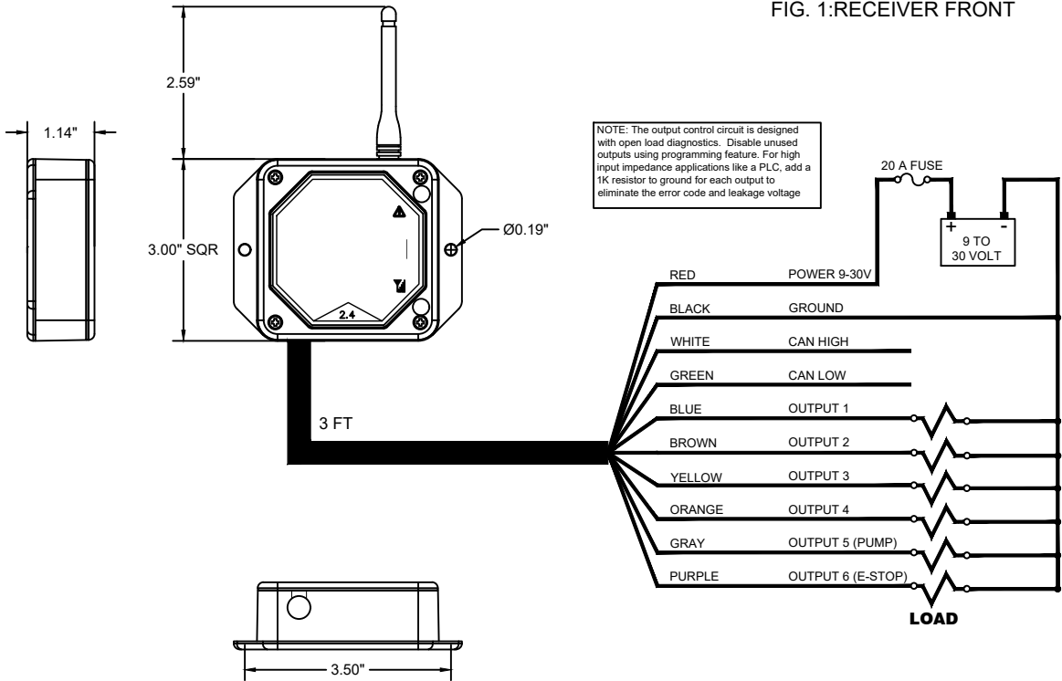
FIG. 1:RECEIVER FRONT
