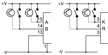
Ingressi Source (PNP)
