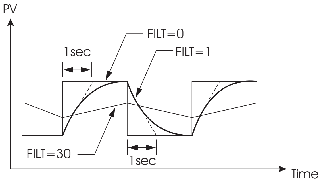
Figure 3-2 Filter Characteristics
