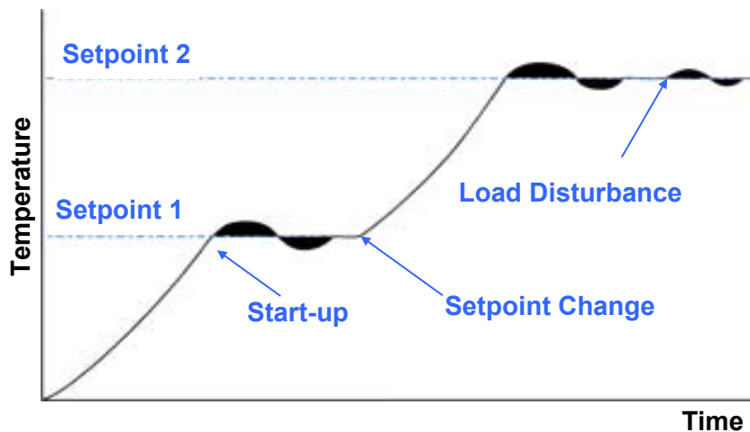
Figure 58. Self-Tune Operation
