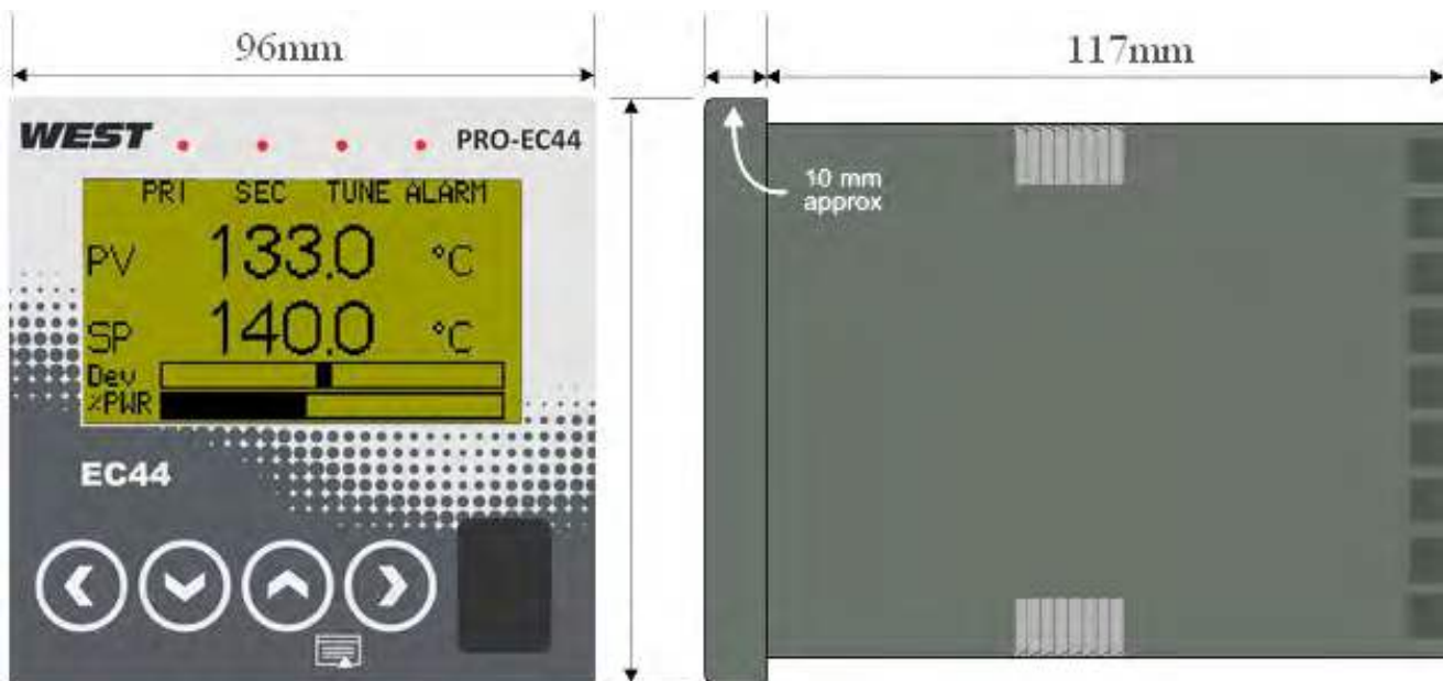
Figure 1. Main dimensions
